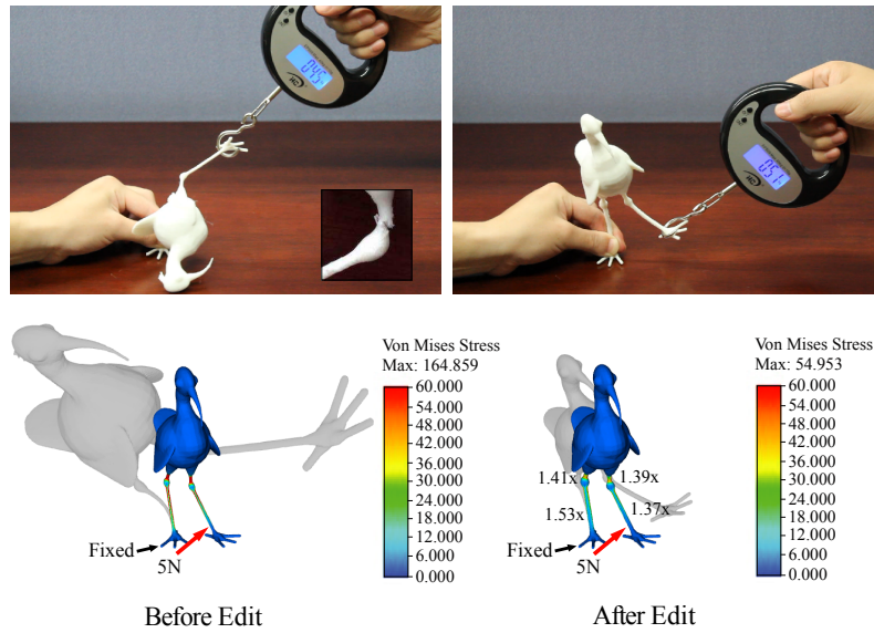
Figure 7: Bird experiment. Left: the object printed from the unedited model broke when a 5N force was exerted on the leg, as predicted by our system. Right: after optimization, the printed object survived the physical experiment. The larger ones of the two optimized scaling factors of each leg domain are marked on the figure.
