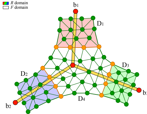
Figure 2: Domain Decomposition. D_1 (red), D_2 (blue) and D_3 (green) are type \mathcal{R} domains and are associated with bones b_1 , b_2 and b_3 respectively. D_4 (white) is a type \mathcal{F} domain adjacent to D_1 , D_2 and D_3 , and is associated with b_1 , b_2 and b_3 simultaneously. The orange points represent vertices on the interface between domains and are duplicated into the domains on both sides.
