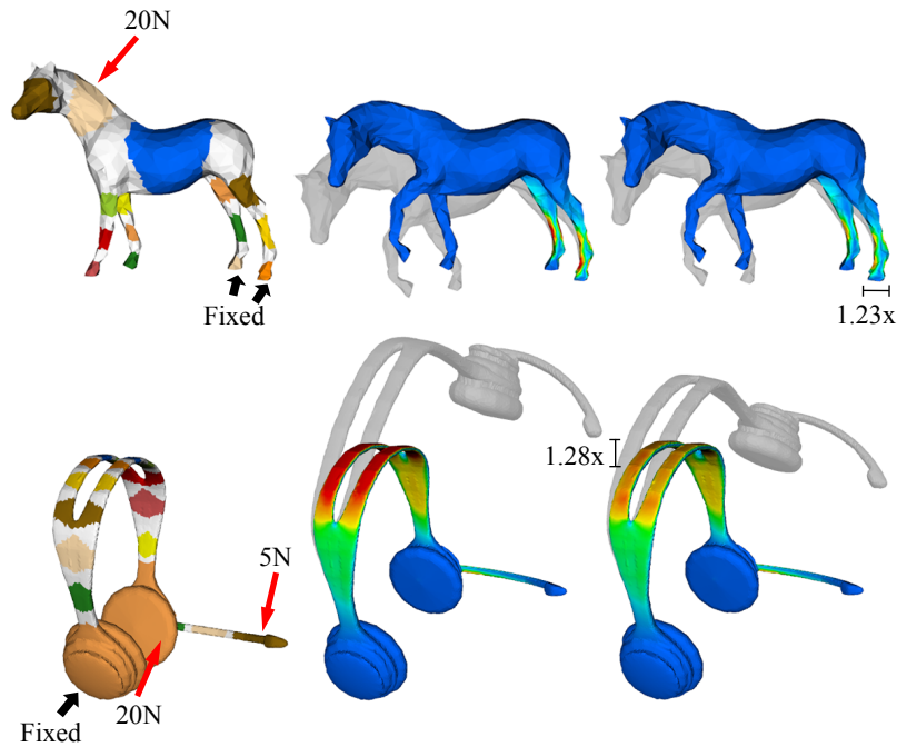
Figure 8: More scenes. Left: domain decompositions and load configurations. Middle: shape editing results, high Von-Mises stresses are presented by red color. Right: meshes after optimization, the maximal scaling are marked on the figure.
