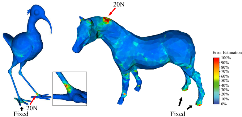
Figure 9: The distribution of the percentage error in energy norm on elements.
