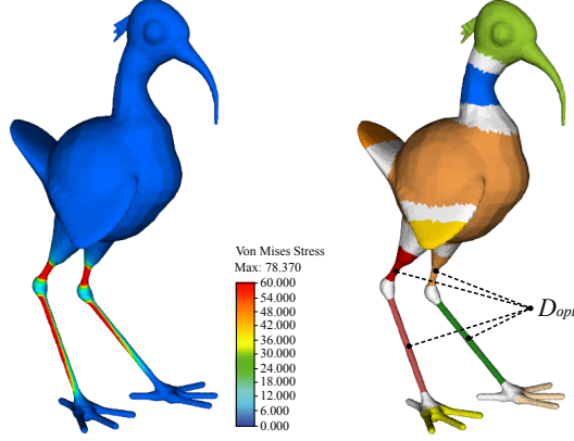
Figure 5: Example of \mathcal{D}_{opt} . Only the four domains having Von-Mises stresses above the threshold ( 60MPa ) are added into \mathcal{D}_{opt} .
