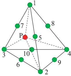
Figure 3: Quadratic tetrahedral element
