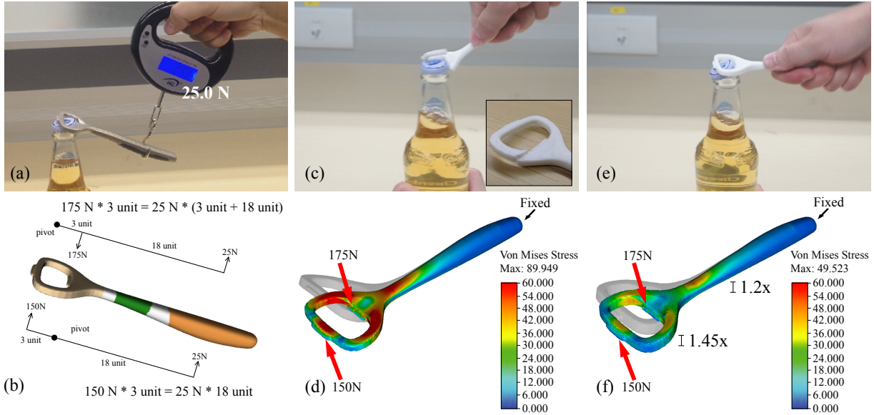
Figure 6: Opener experiment. (a, b) We measured the loads with an electric spring scale. The magnitude of the forces exerted on different parts of the opener are computed by torque equilibrium. (c, d) Before editing, our system predicted that the maximal Von-Mises stress in the model exceeded the yielding strength of the material, and the printed object broke in the experiment. (e, f) After editing, our system predicted that the high stresses had been reduced, and the printed object survived the experiment.
